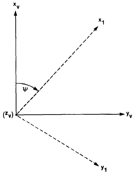
(a) Rotation through \psi about z_v axis.
