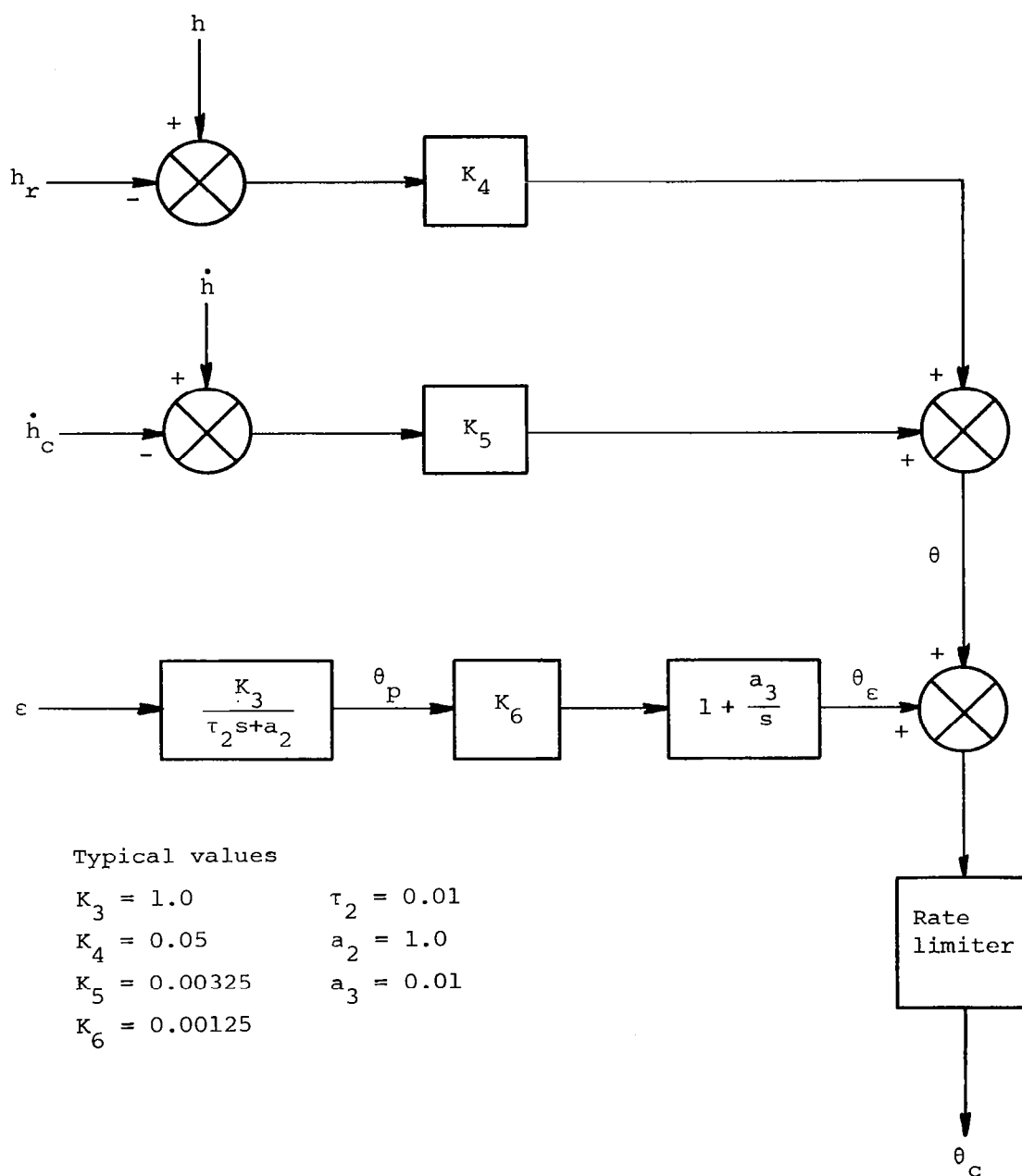
Figure 15 Glide slope tracking mode
